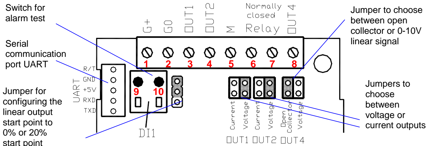
Figure 3. The connection terminal area of the aSENSE® m III with jumpers and terminals. The terminal DI1 may be used for forced ventilation. If the sensor has a heater it is connected to G+ and G0.
