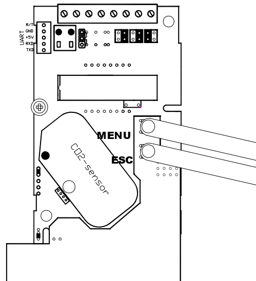
Figure 7. The ENTER command is done by pushing buttons MENU and ESC at the same time for about 14 seconds
