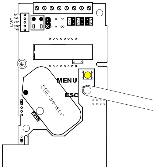
Figure 6. The push button MENU is pushed
