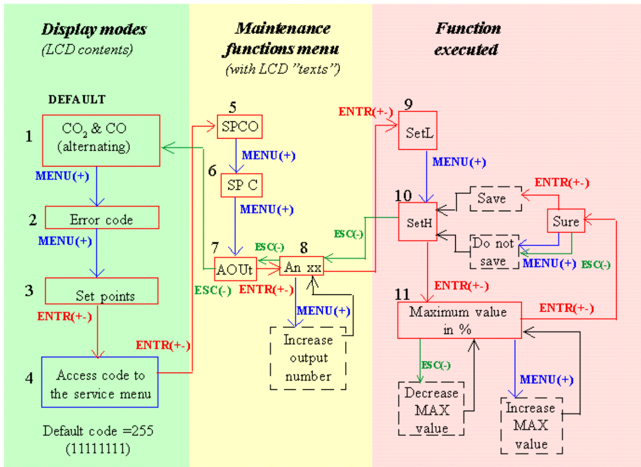
Figure 8. Maintenance functions available on aSENSE ® m III to set output limits. Only flow chart for setting High limits are shown, but Low limits are set in the very same way. The numbers in the flow chart refers to the points in example 1. Function blocks that are time limited are indicated by blue borders. Time limit refers to an internal time-out that returns the LCD and maintenance function back to normal. ENTER is a simultaneous pressing on MENU and ESC.
