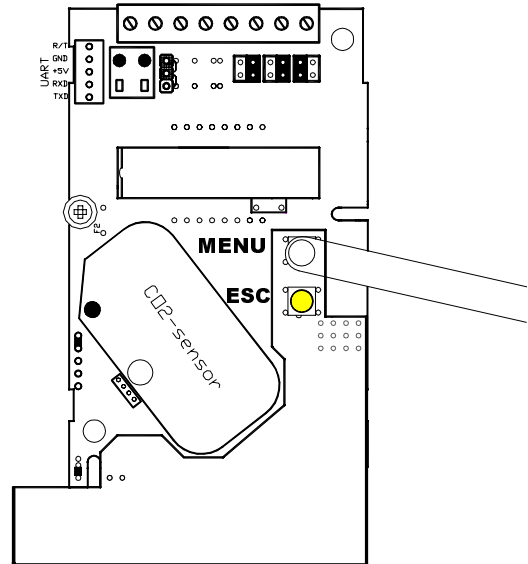
Figure 5. The push button MENU is pushed
