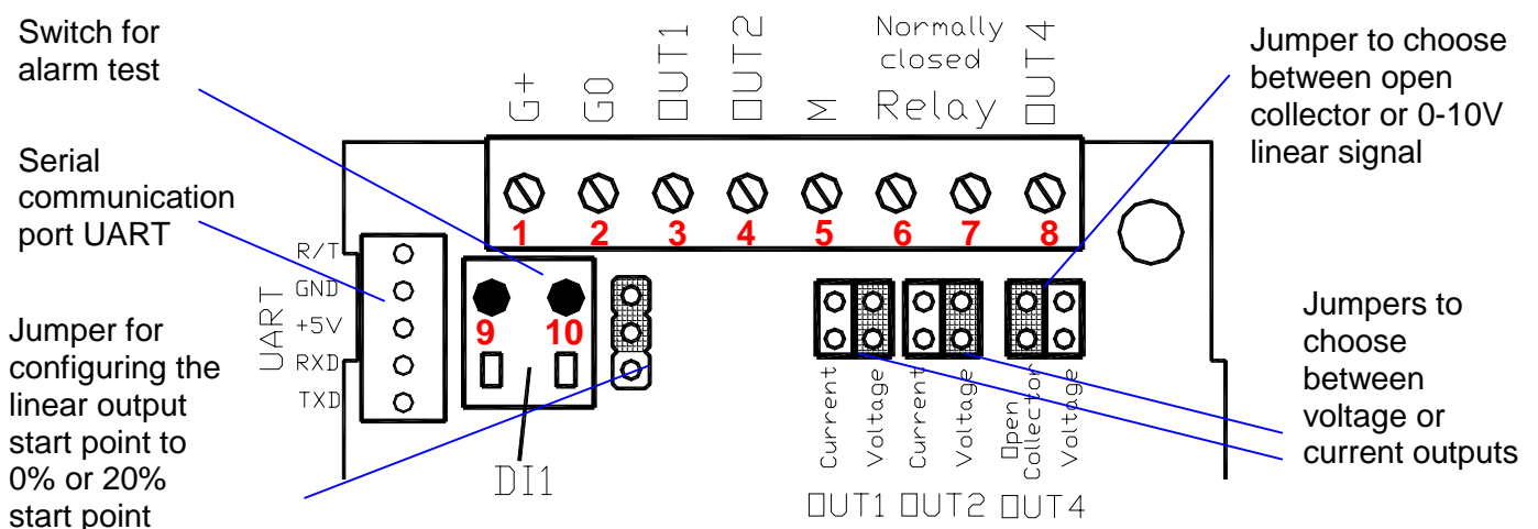
Figure 9. The aSENSE® m III printed circuit board with the connection terminal area is enlarged. The terminal DI1 may be used for forced ventilation. If the sensor has a heater it is connected to G+ and G0.
