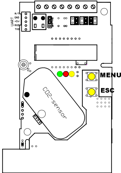
Figure 4. The sensor with push buttons
