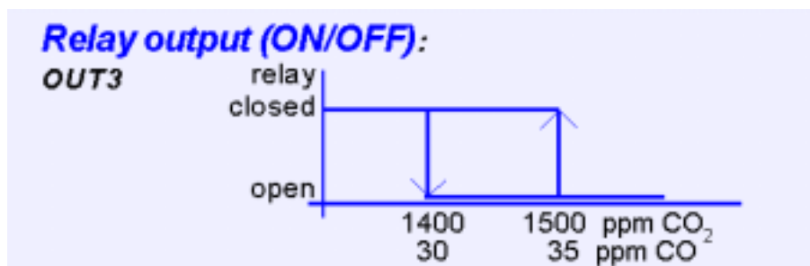
Figure 2. The control signal of air quality
